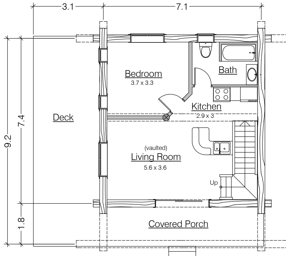
Main Floor Plan 55.7 Sq. M.
