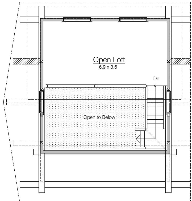
Loft Floor Plan 26.0 Sq. M.
